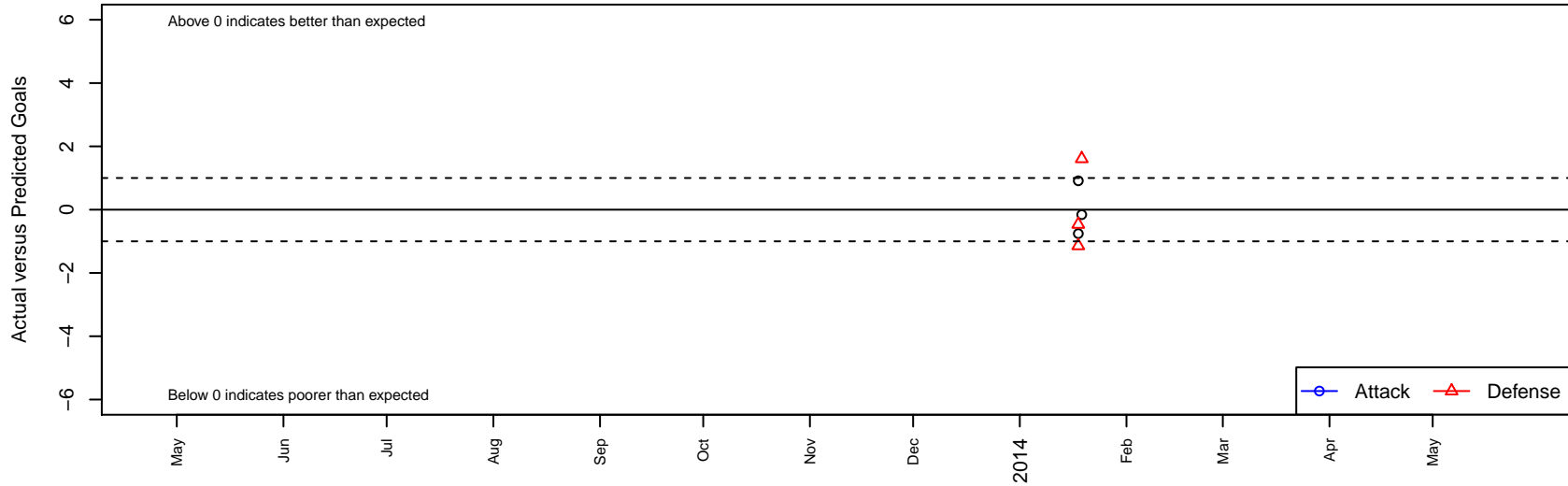
Arizona Hammers 02 Chavez G01 Dots are actual minus expected GF (blue circles) and GA (red triangles). Blue line is smoothed change in attack strength. Red is smoothed change in defense strength.
